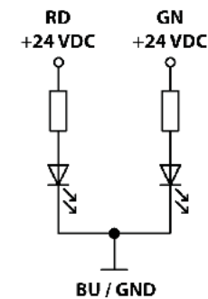
Wiring Diagram
