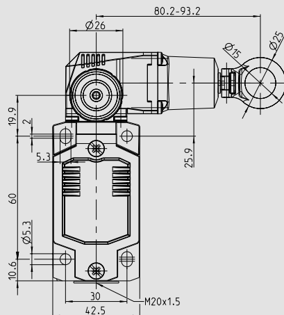
SRO-M78...HR...-2
