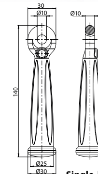
Single-handle
